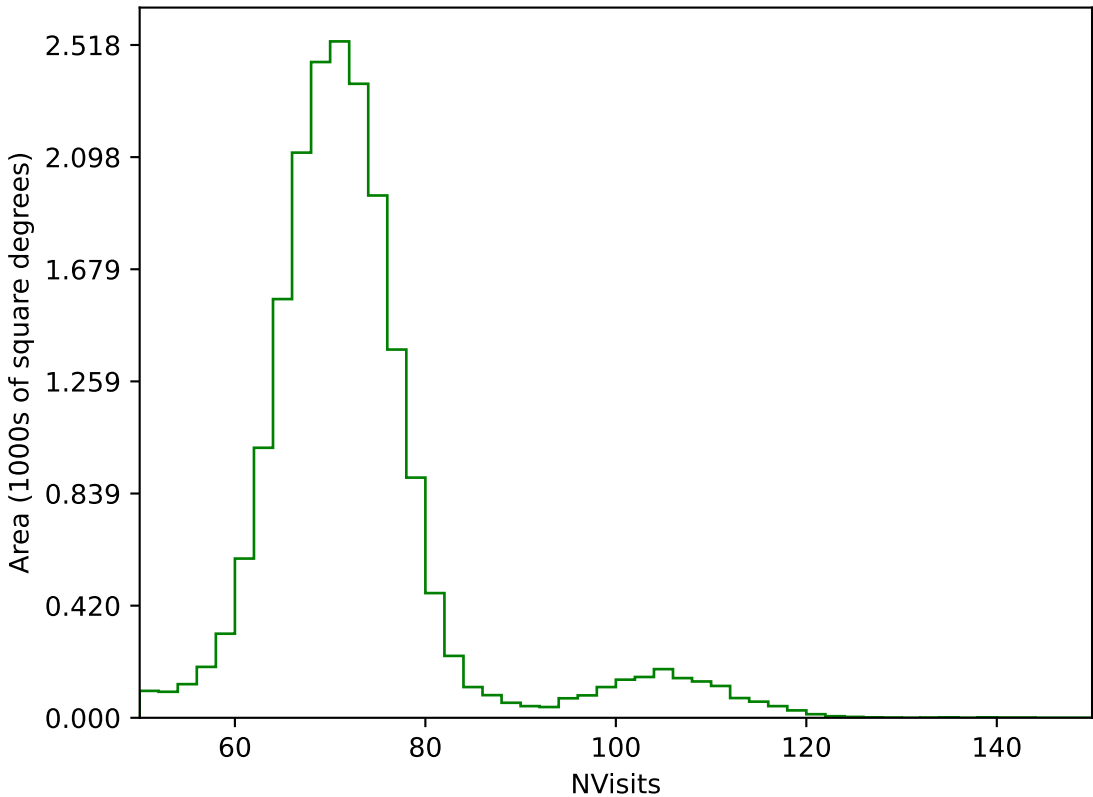
internal_u_expt30_nscale0.9v3.4_10yrs All sky g band: NVisits
