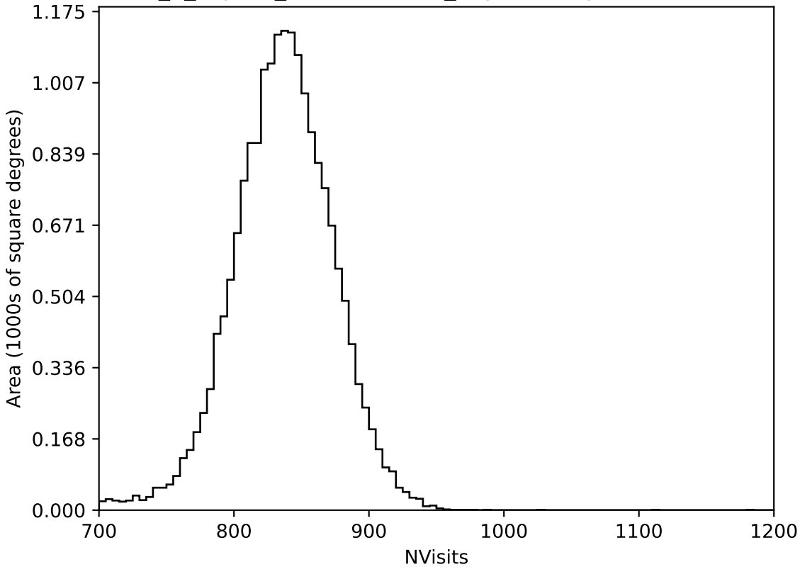
internal_u_expt30_nscale0.9v3.4_10yrs All sky all bands: NVisits
