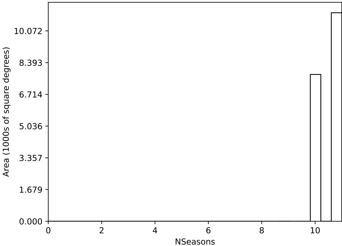
internal_u_expt30_nscale0.9v3.4_10yrs WFD all bands: NSeasons
