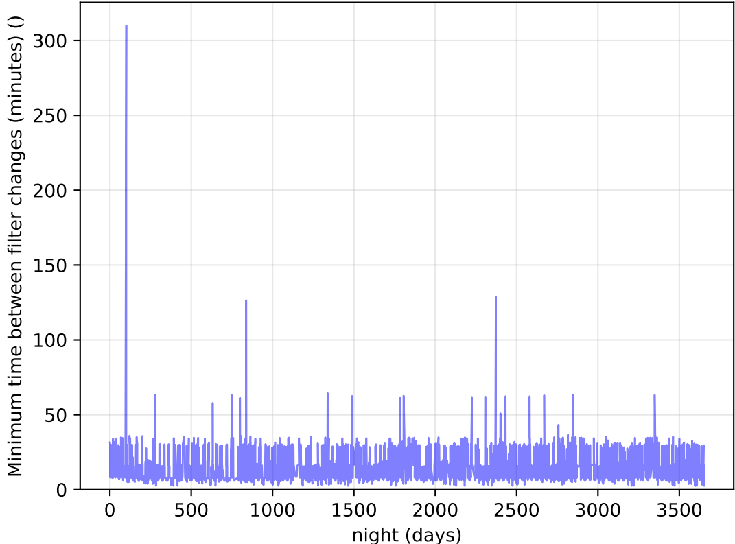
internal_u_expt30_nscale0.9v3.4_10yrs Per Night: Minimum time between filter changes (minutes)
