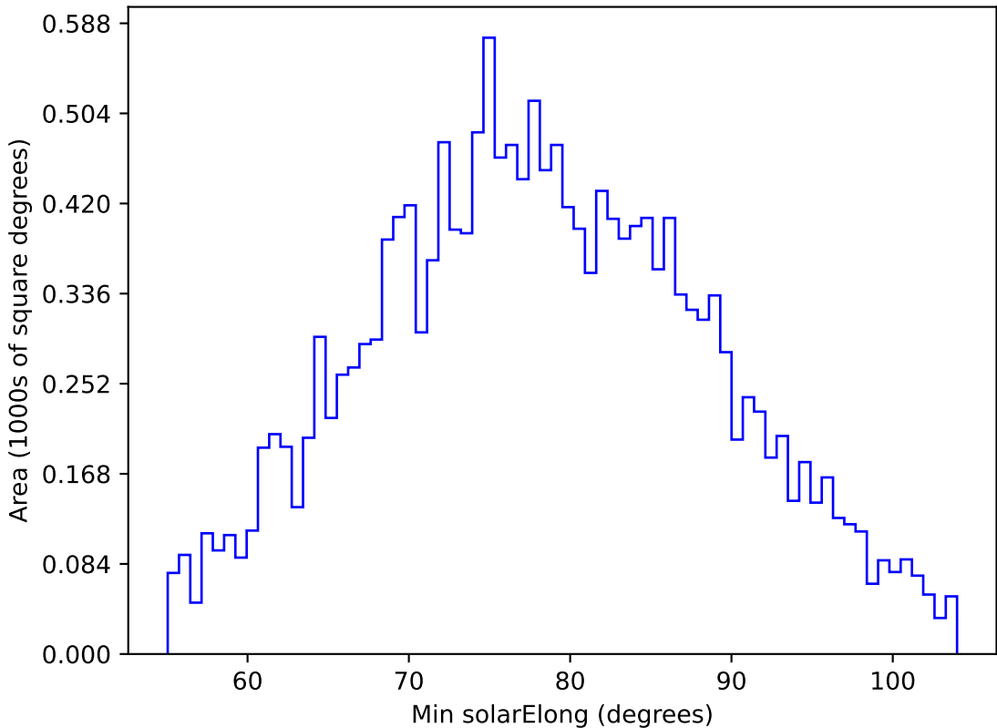
internal_u_expt30_nscale0.9v3.4_10yrs WFD u band: Min solarElong
