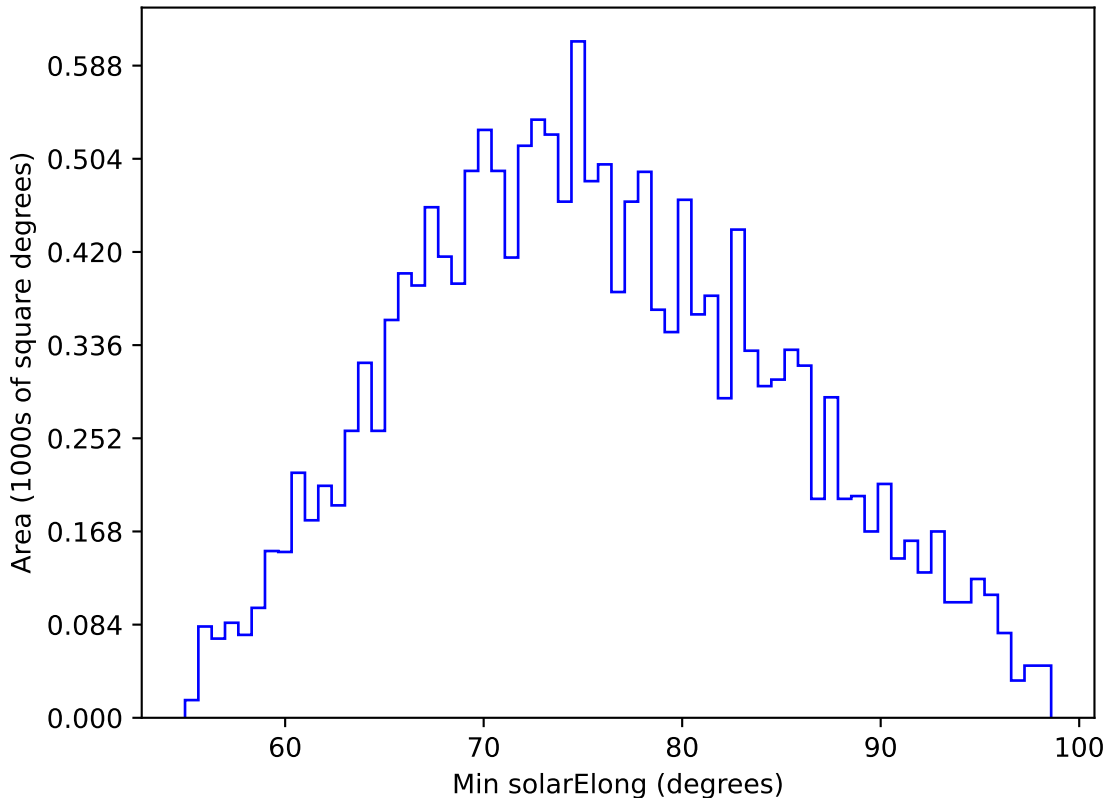
internal_u_expt30_nscale0.9v3.4_10yrs WFD g band: Min solarElong
