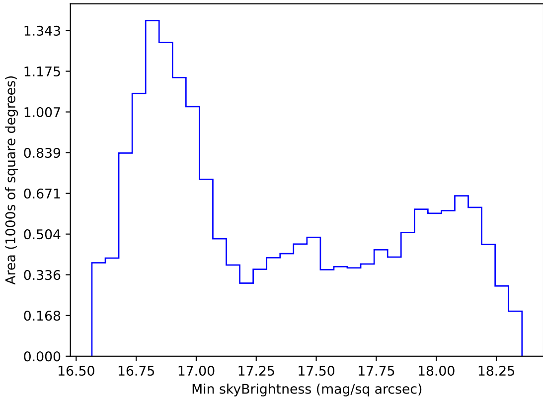
internal_u_expt30_nscale0.9v3.4_10yrs WFD z band: Min skyBrightness
