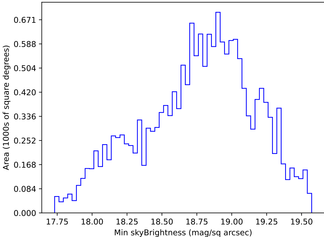
internal_u_expt30_nscale0.9v3.4_10yrs WFD r band: Min skyBrightness
