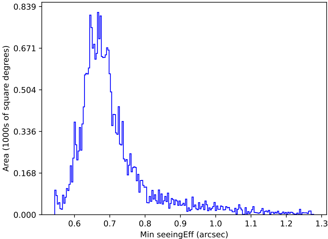
internal_u_expt30_nscale0.9v3.4_10yrs Yr 1 i band: Min seeingEff
