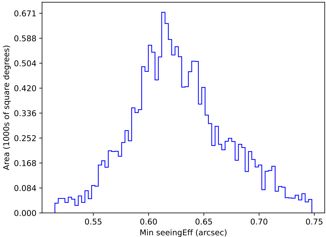
internal_u_expt30_nscale0.9v3.4_10yrs WFD y band: Min seeingEff
