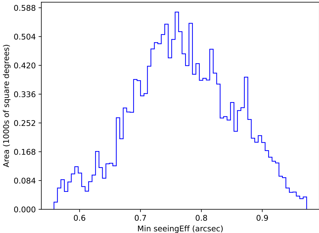
internal_u_expt30_nscale0.9v3.4_10yrs WFD u band: Min seeingEff
