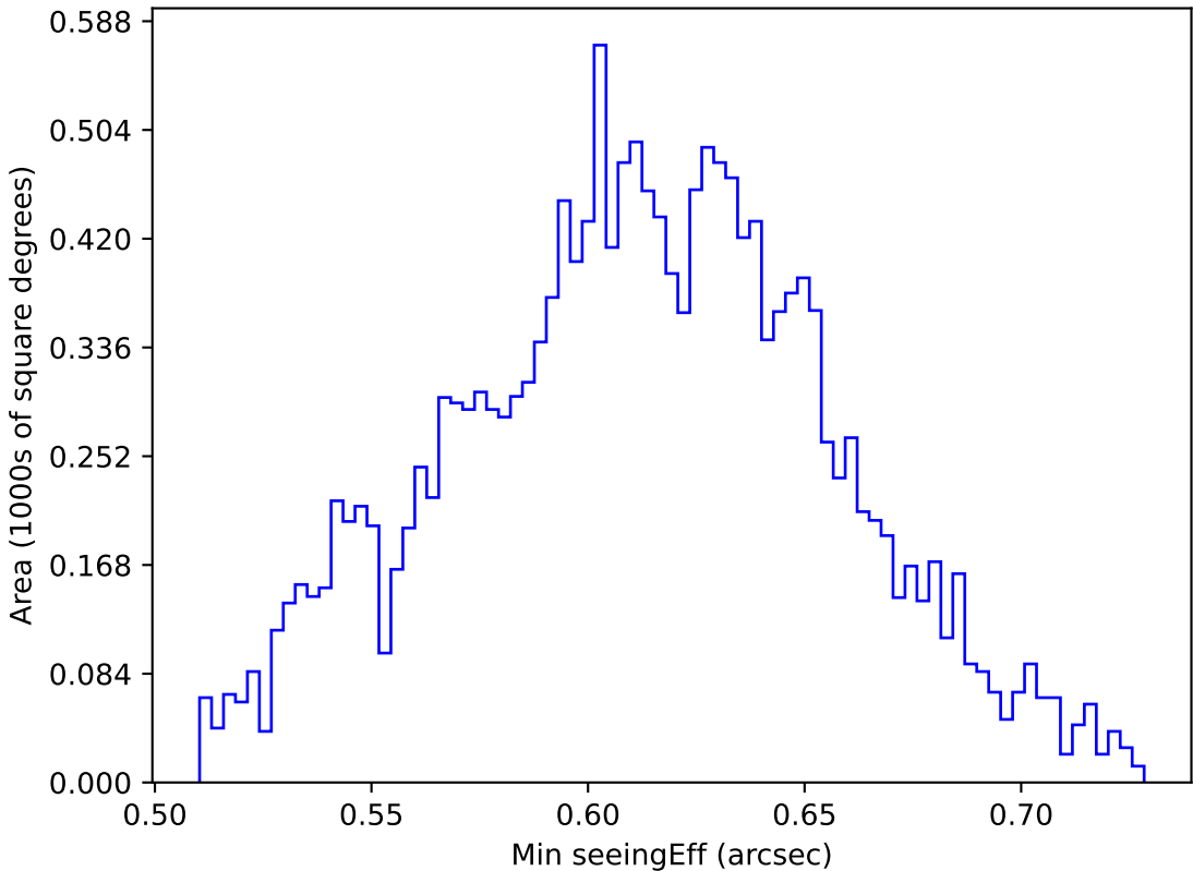
internal_u_expt30_nscale0.9v3.4_10yrs WFD r band: Min seeingEff
