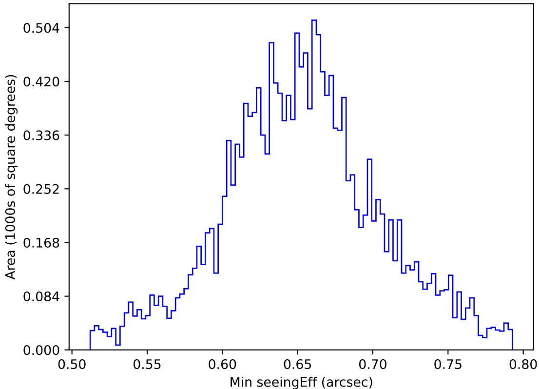
internal_u_expt30_nscale0.9v3.4_10yrs WFD g band: Min seeingEff
