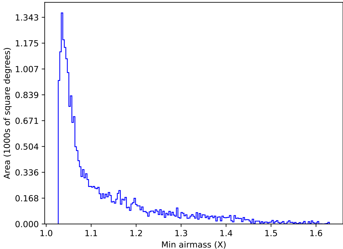
internal_u_expt30_nscale0.9v3.4_10yrs Yr 1 y band: Min airmass
