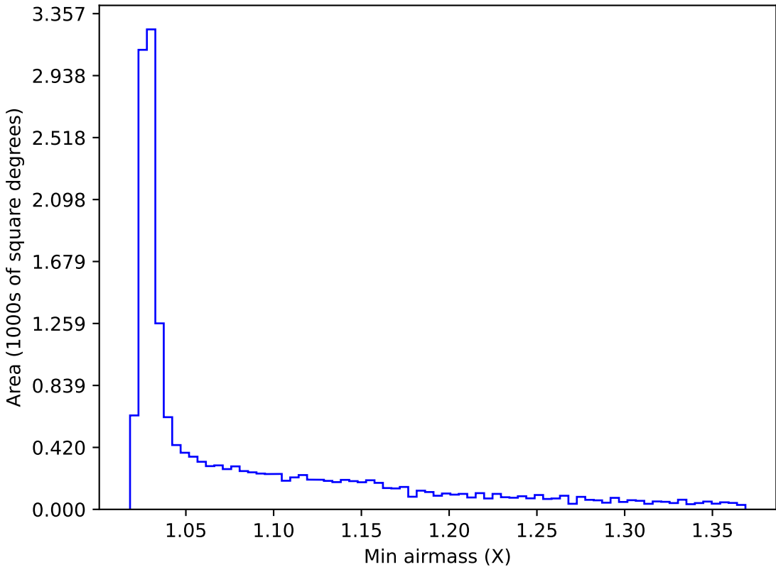
internal_u_expt30_nscale0.9v3.4_10yrs WFD z band: Min airmass
