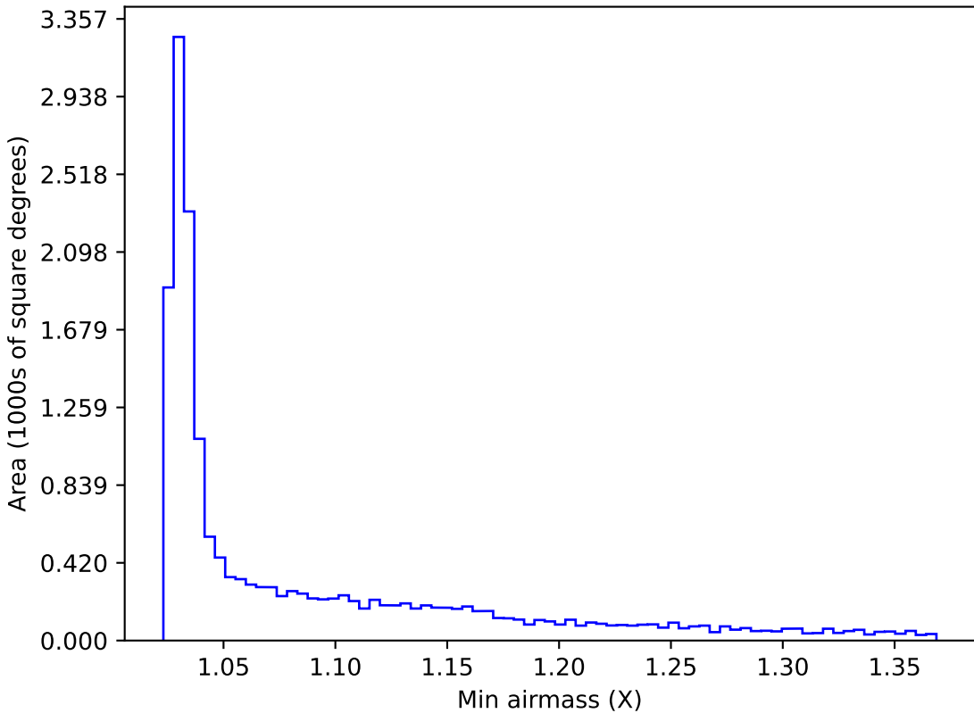
internal_u_expt30_nscale0.9v3.4_10yrs WFD y band: Min airmass
