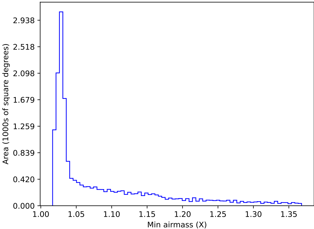
internal_u_expt30_nscale0.9v3.4_10yrs WFD r band: Min airmass
