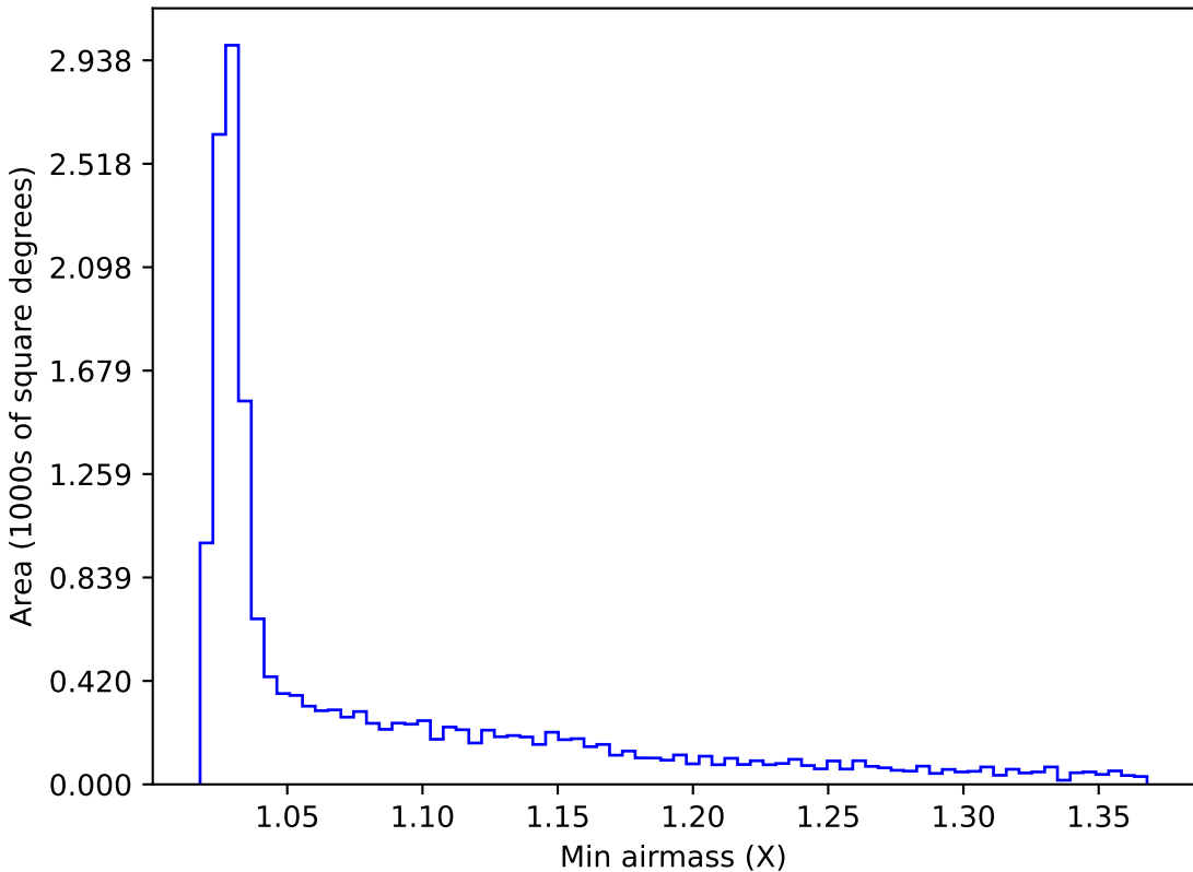
internal_u_expt30_nscale0.9v3.4_10yrs WFD i band: Min airmass
