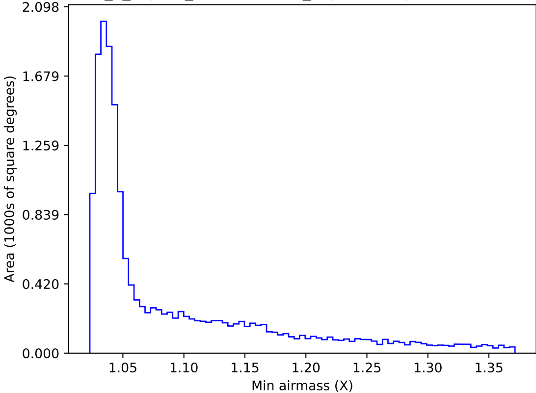
internal_u_expt30_nscale0.9v3.4_10yrs WFD g band: Min airmass
