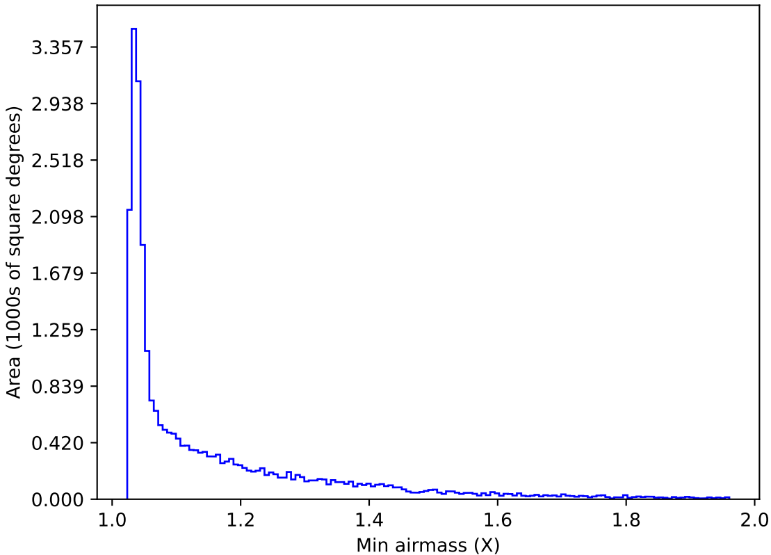
internal_u_expt30_nscale0.9v3.4_10yrs All sky g band: Min airmass
