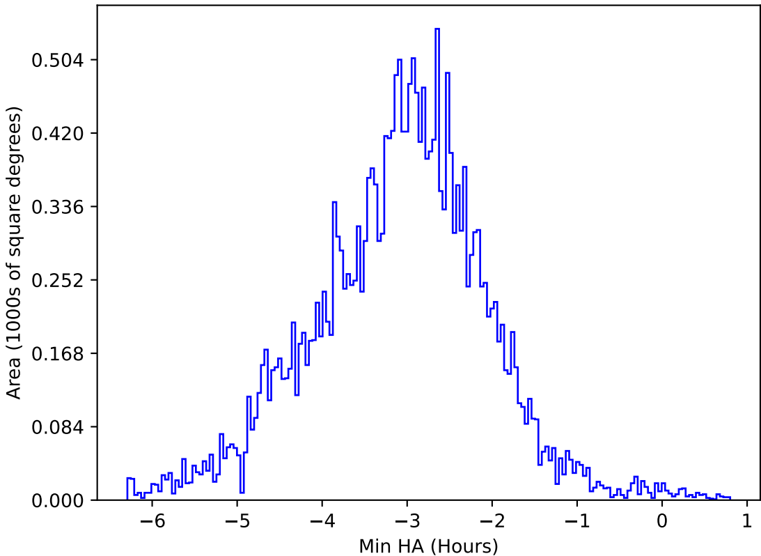
internal_u_expt30_nscale0.9v3.4_10yrs All sky u band: Min HA
