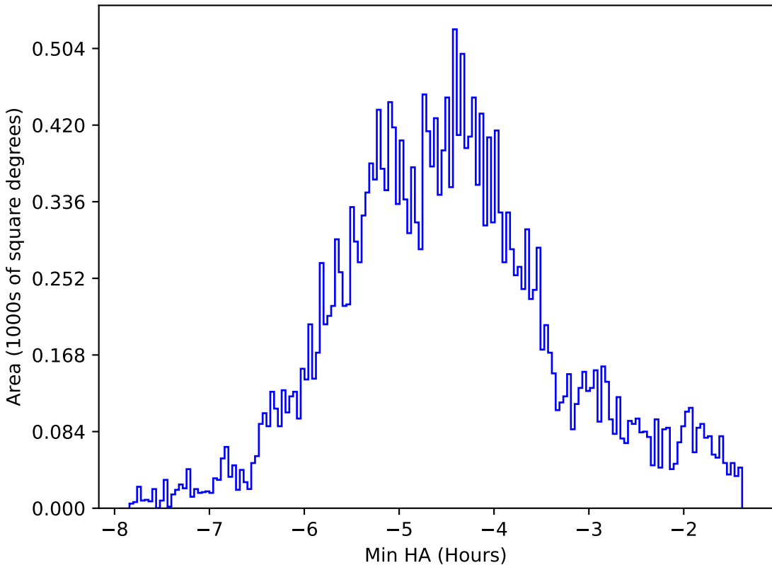
internal_u_expt30_nscale0.9v3.4_10yrs All sky all bands: Min HA
