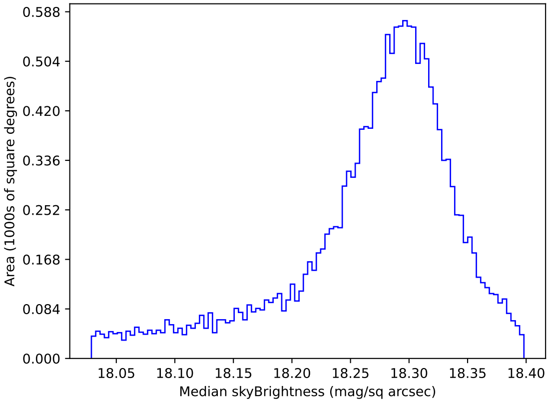
internal_u_expt30_nscale0.9v3.4_10yrs WFD y band: Median skyBrightness
