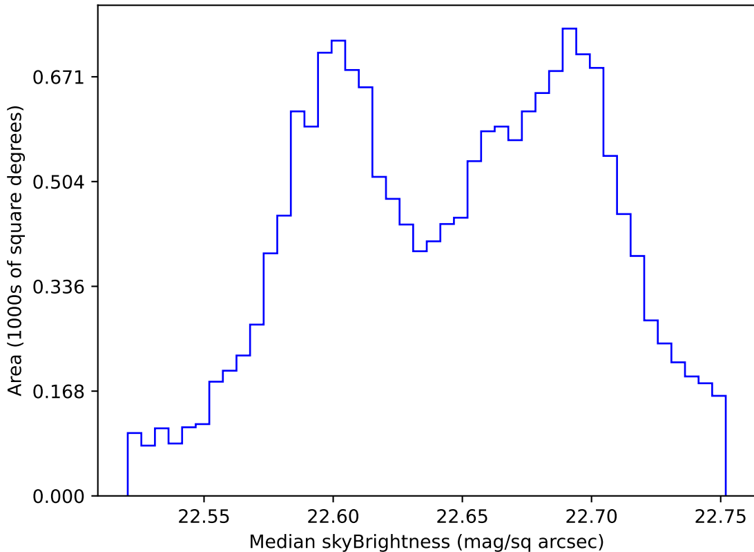
internal_u_expt30_nscale0.9v3.4_10yrs WFD u band: Median skyBrightness
