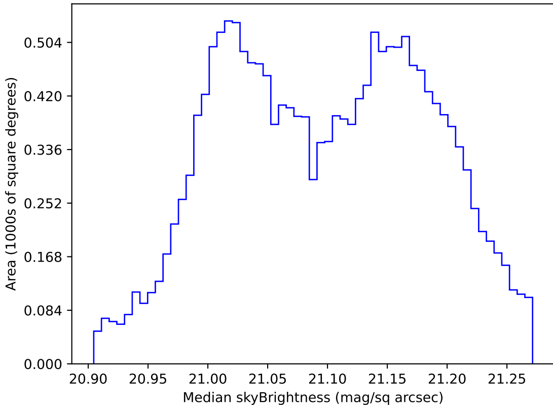
internal_u_expt30_nscale0.9v3.4_10yrs WFD r band: Median skyBrightness
