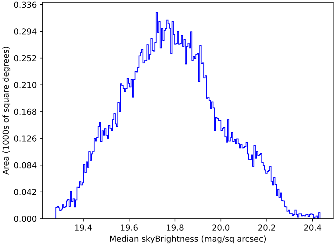
internal_u_expt30_nscale0.9v3.4_10yrs All sky all bands: Median skyBrightness
