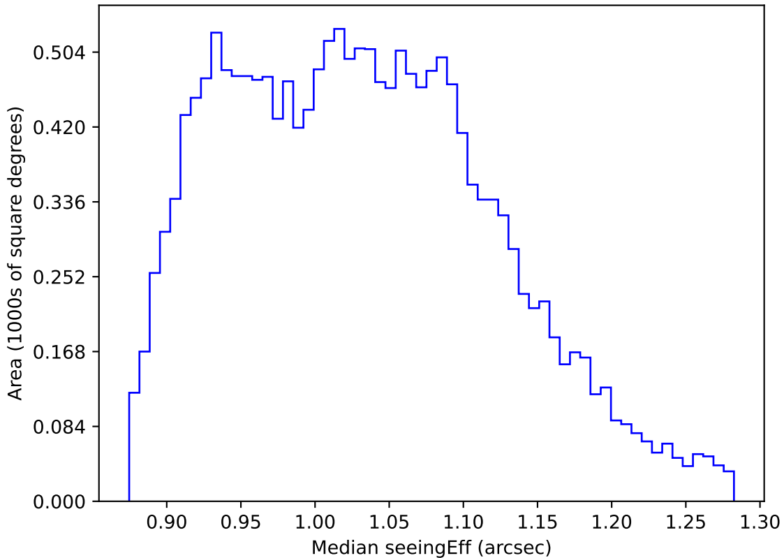
internal_u_expt30_nscale0.9v3.4_10yrs WFD r band: Median seeingEff
