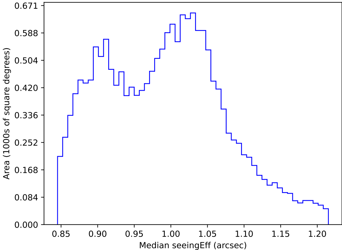
internal_u_expt30_nscale0.9v3.4_10yrs WFD i band: Median seeingEff
