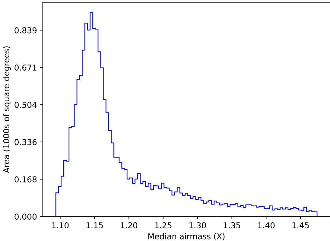
internal_u_expt30_nscale0.9v3.4_10yrs WFD y band: Median airmass
