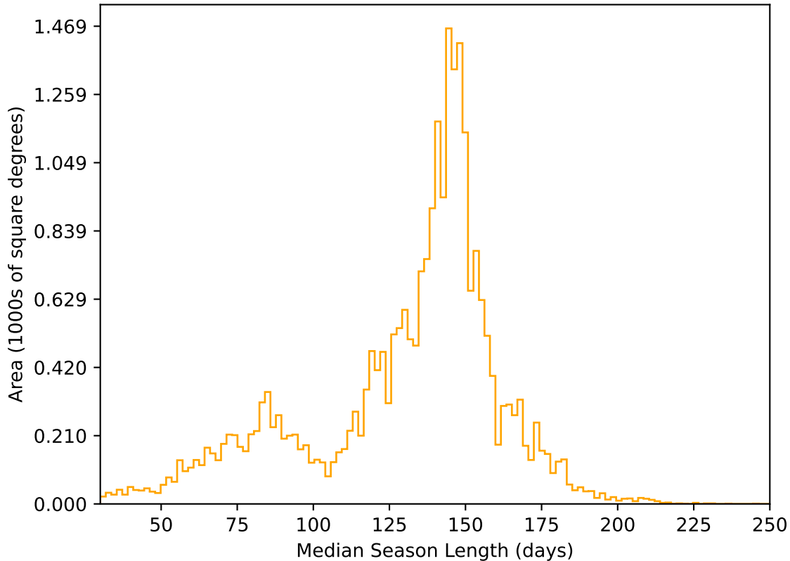
internal_u_expt30_nscale0.9v3.4_10yrs All sky r band: Median Season Length
