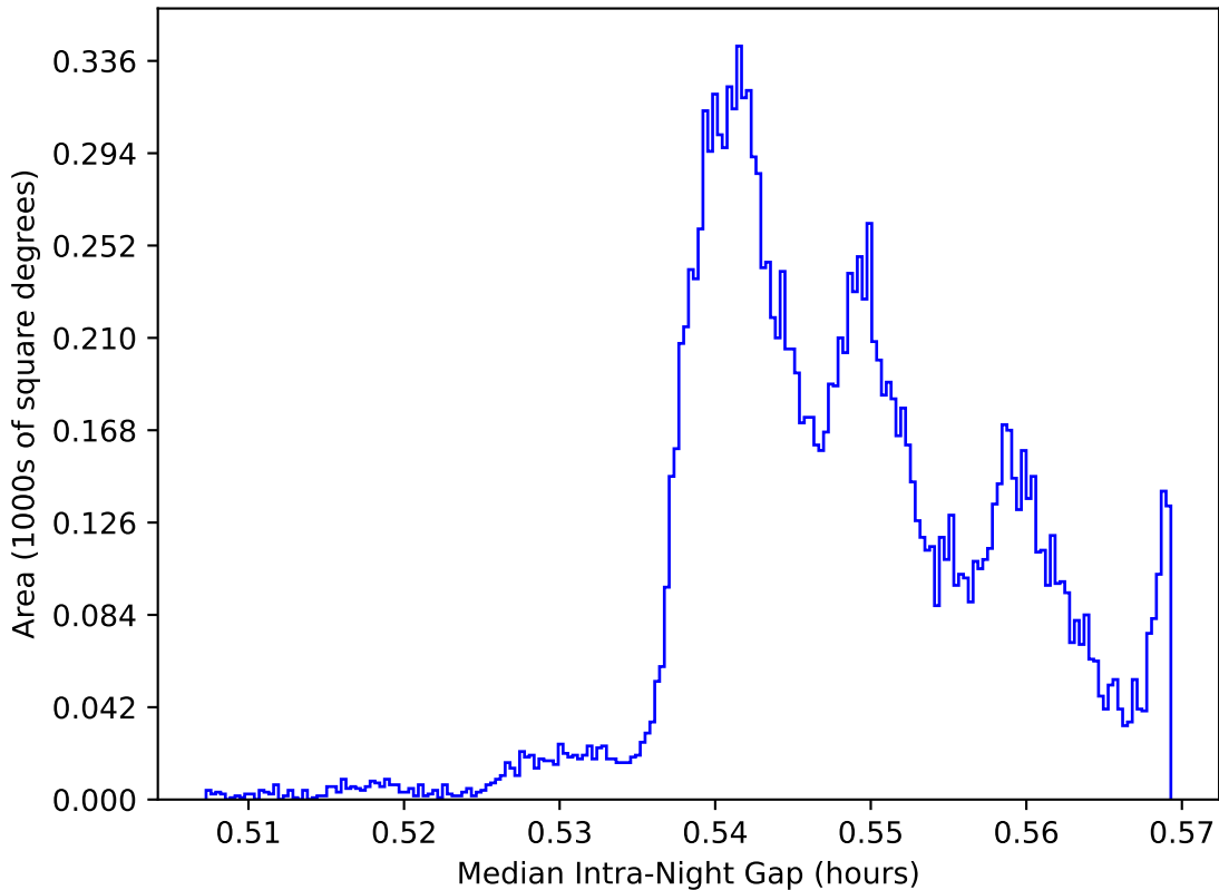
internal_u_expt30_nscale0.9v3.4_10yrs WFD: Median Intra-Night Gap
