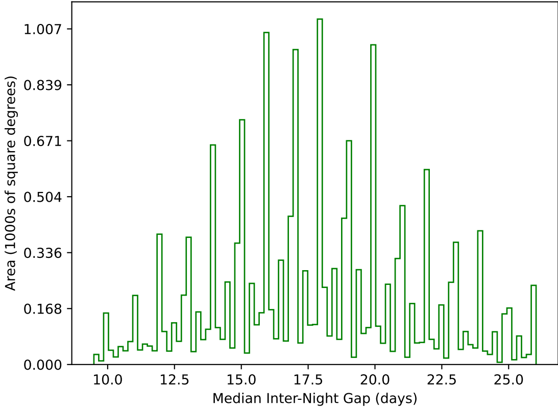
internal_u_expt30_nscale0.9v3.4_10yrs WFD g band: Median Inter-Night Gap
