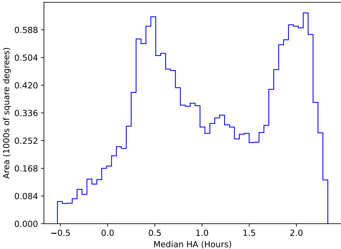
internal_u_expt30_nscale0.9v3.4_10yrs WFD z band: Median HA
