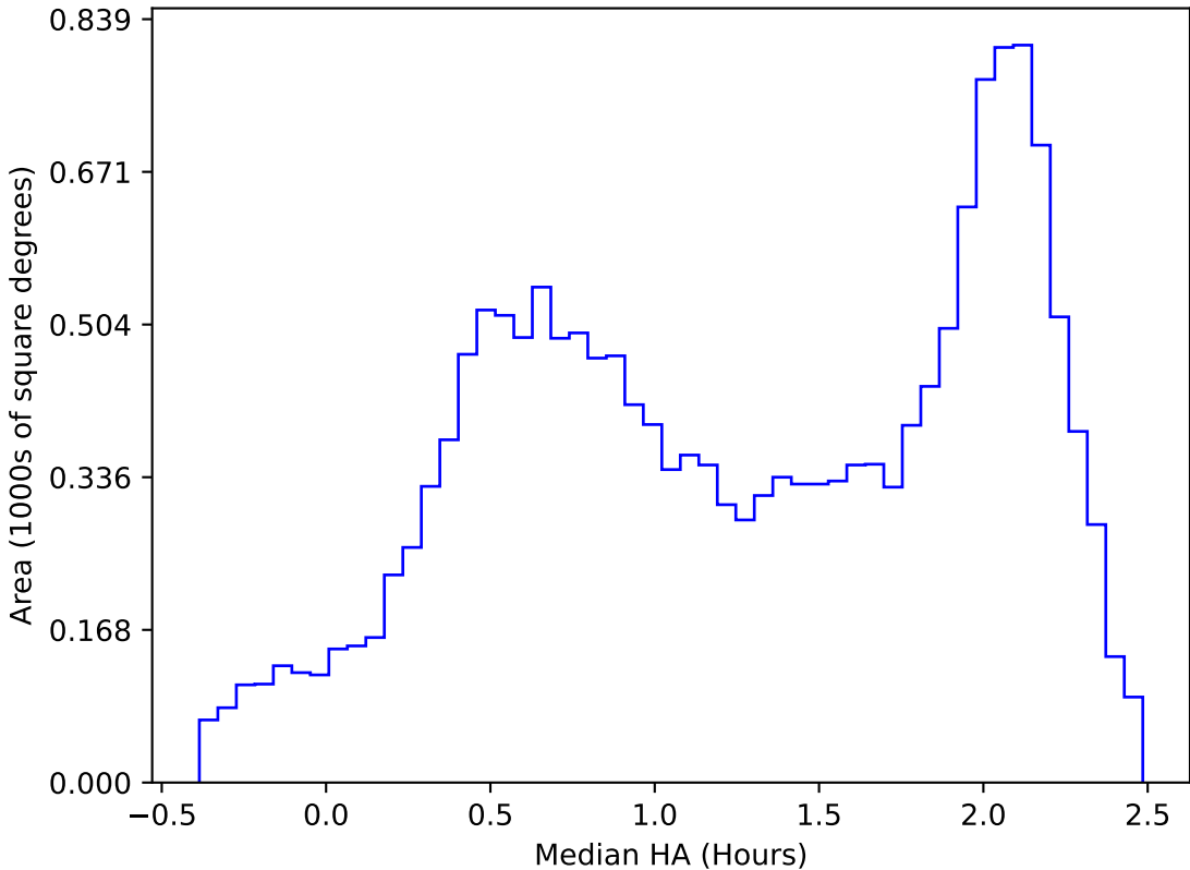
internal_u_expt30_nscale0.9v3.4_10yrs WFD y band: Median HA
