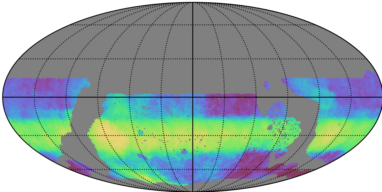
internal_u_expt30_nscale0.9v3.4_10yrs WFD r band: Median HA
