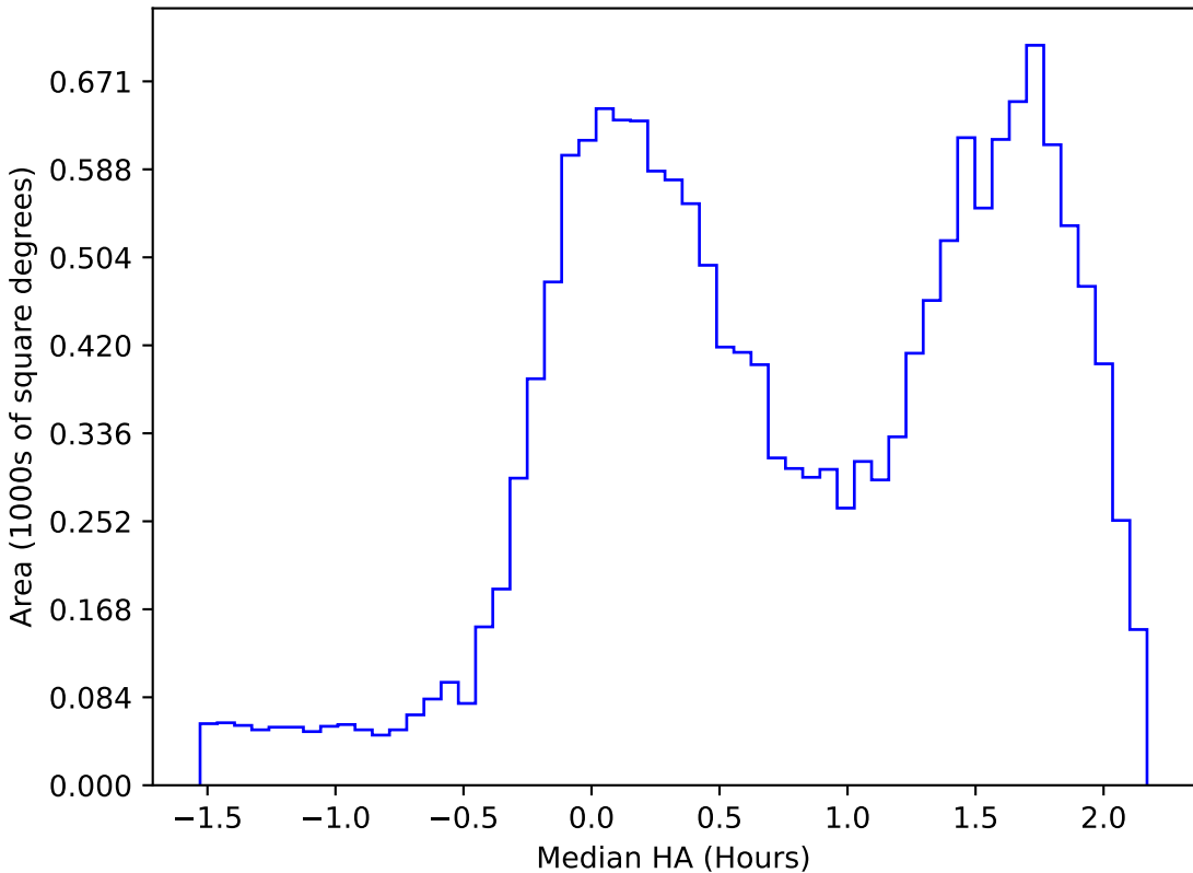
internal_u_expt30_nscale0.9v3.4_10yrs WFD g band: Median HA
