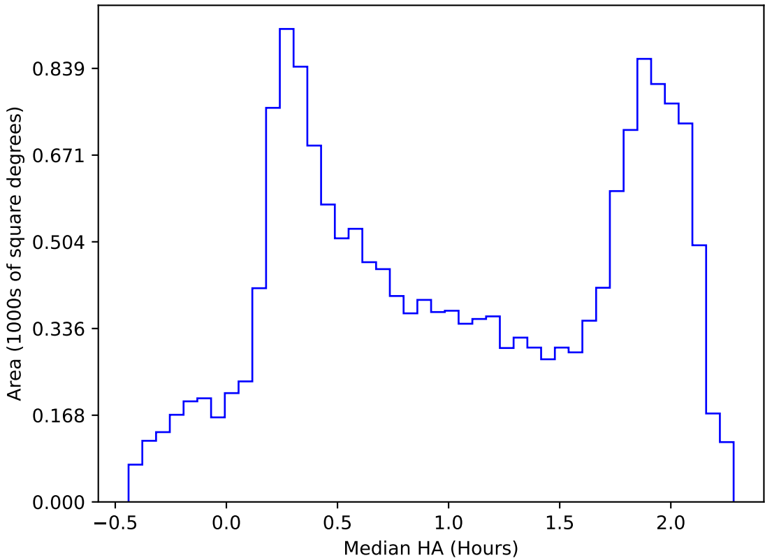
internal_u_expt30_nscale0.9v3.4_10yrs WFD all bands: Median HA
