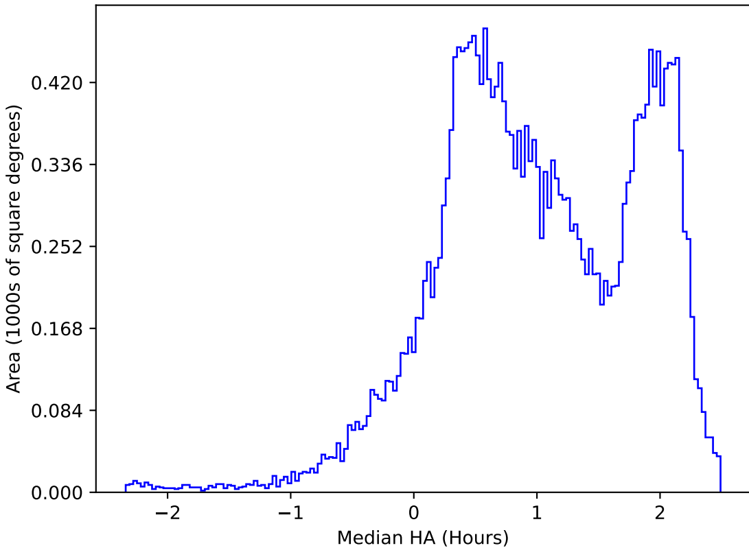
internal_u_expt30_nscale0.9v3.4_10yrs All sky z band: Median HA
