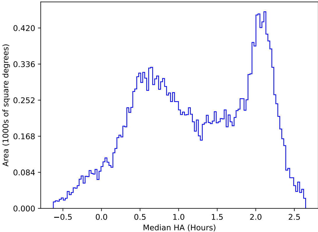
internal_u_expt30_nscale0.9v3.4_10yrs All sky y band: Median HA
