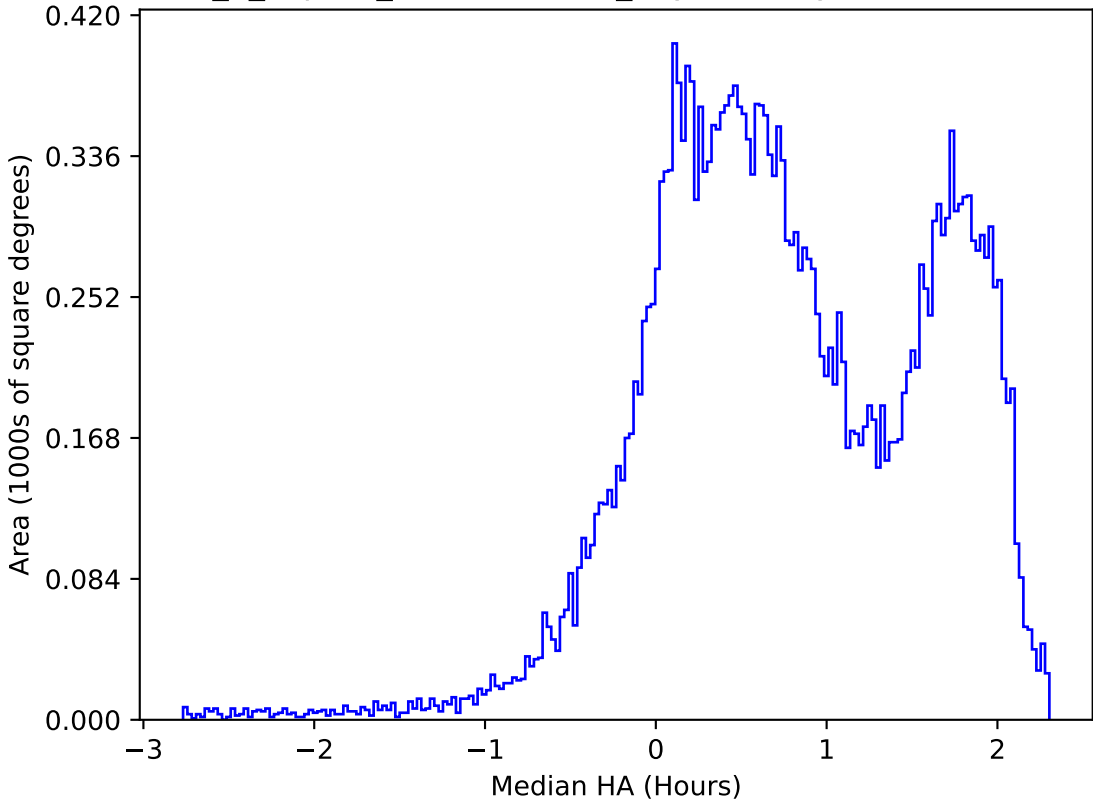
internal_u_expt30_nscale0.9v3.4_10yrs All sky r band: Median HA
