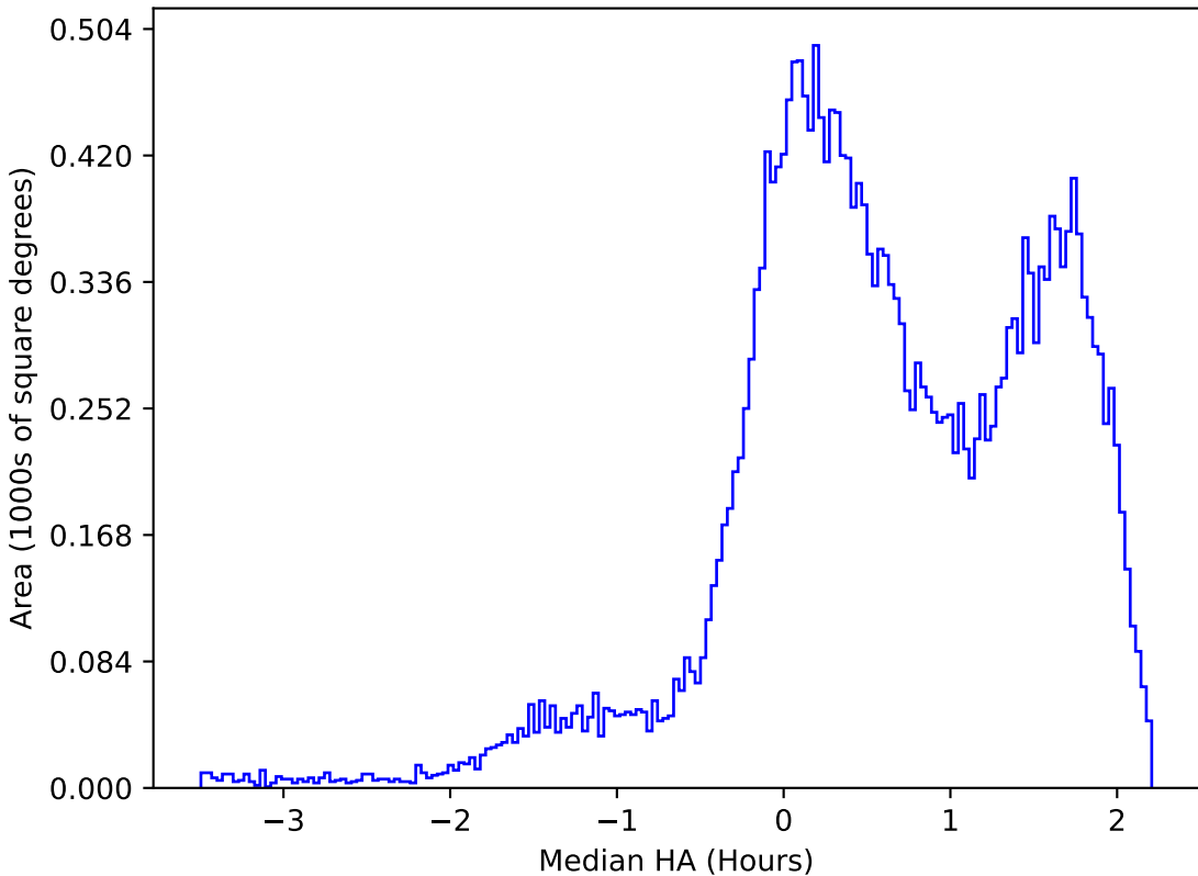
internal_u_expt30_nscale0.9v3.4_10yrs All sky g band: Median HA
