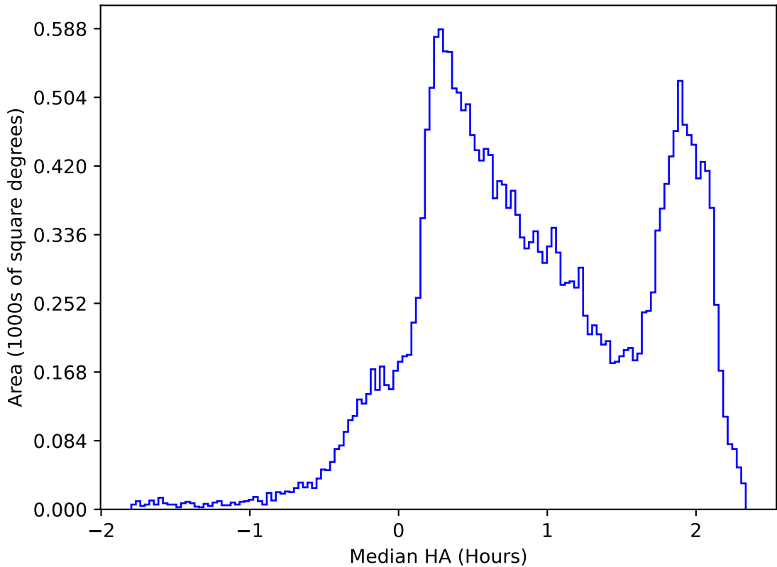
internal_u_expt30_nscale0.9v3.4_10yrs All sky all bands: Median HA
