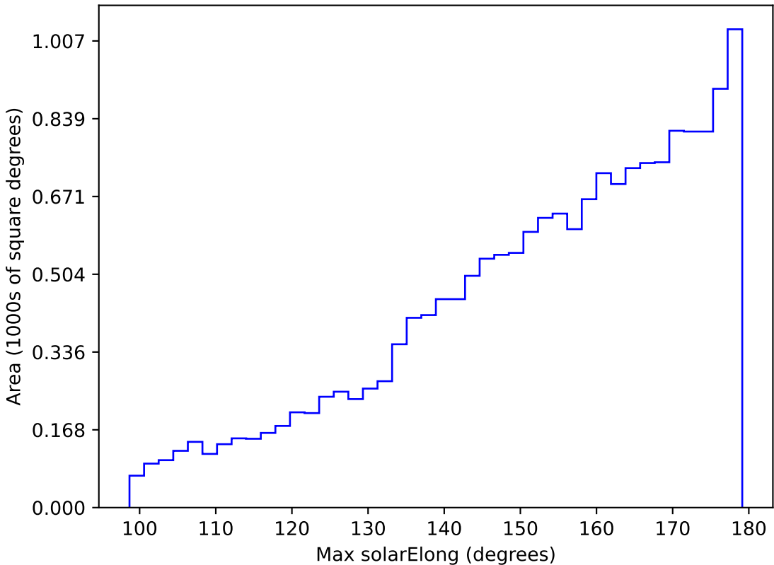
internal_u_expt30_nscale0.9v3.4_10yrs WFD y band: Max solarElong
