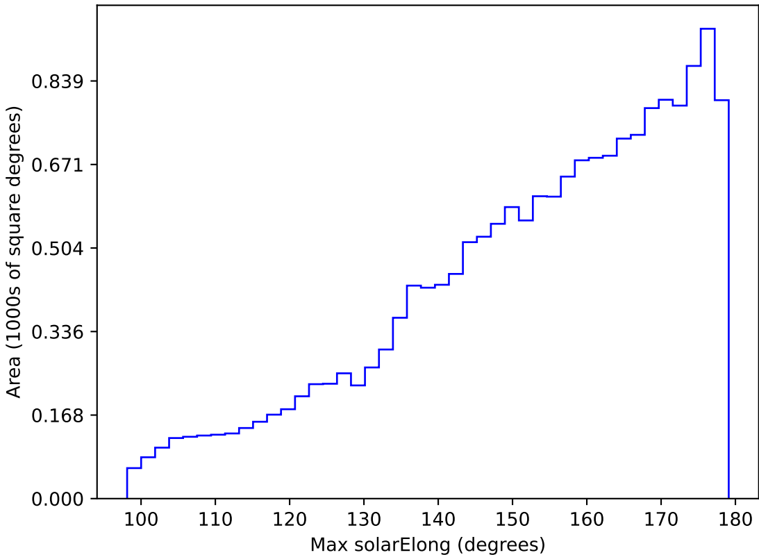
internal_u_expt30_nscale0.9v3.4_10yrs WFD g band: Max solarElong
