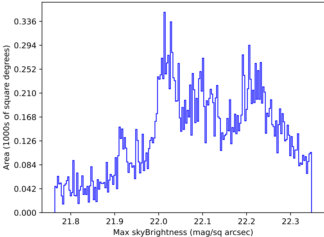
internal_u_expt30_nscale0.9v3.4_10yrs Yr 1 g band: Max skyBrightness
