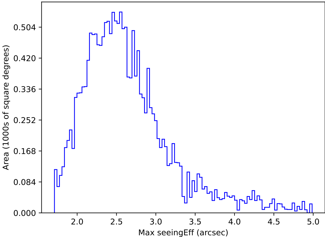
internal_u_expt30_nscale0.9v3.4_10yrs WFD z band: Max seeingEff
