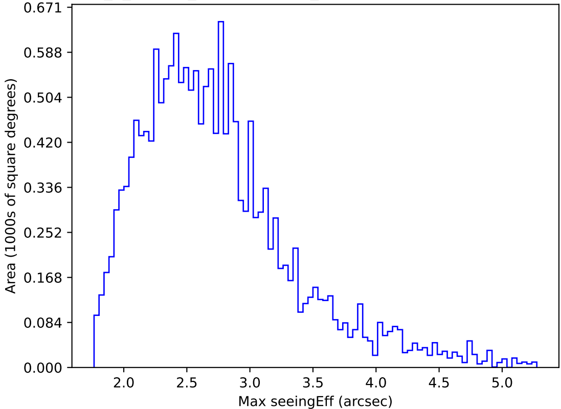
internal_u_expt30_nscale0.9v3.4_10yrs WFD i band: Max seeingEff
