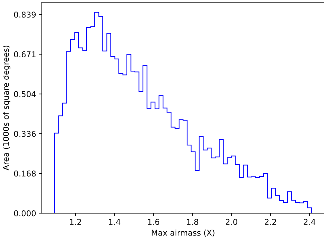
internal_u_expt30_nscale0.9v3.4_10yrs Yr 1 u band: Max airmass
