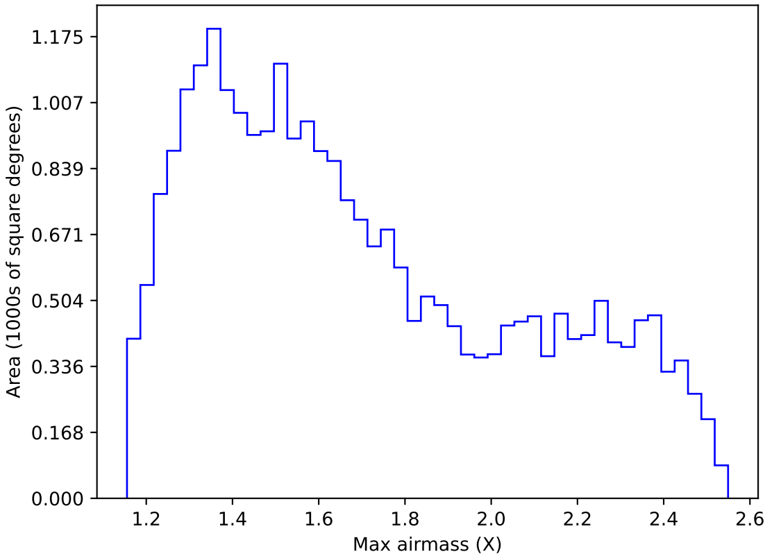
internal_u_expt30_nscale0.9v3.4_10yrs Yr 1 r band: Max airmass
