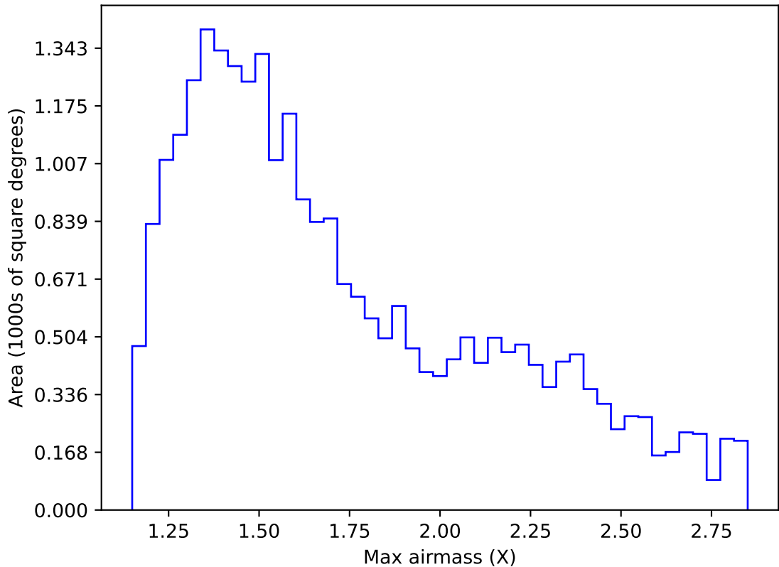
internal_u_expt30_nscale0.9v3.4_10yrs Yr 1 i band: Max airmass
